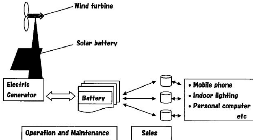
Figure 1 Small lot electric power supply system
