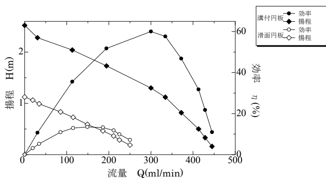
(c) Performance curve
